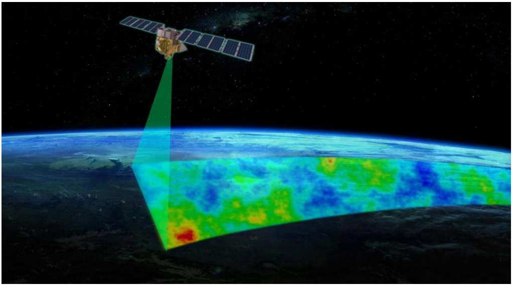
Satellite: ESA Sentinel 5P Instrument: TROPOMI Gas: CH 4 Target: south U
