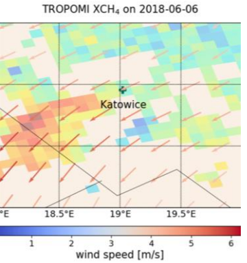
Satellite: ESA Sentinel 5P Instrument: TROPOMI Gas: CH 4 Target: south U
