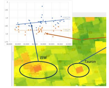
Satellite: ESA Sentinel 5P Instrument: TROPOMI Gas: CH 4 Target: south U
